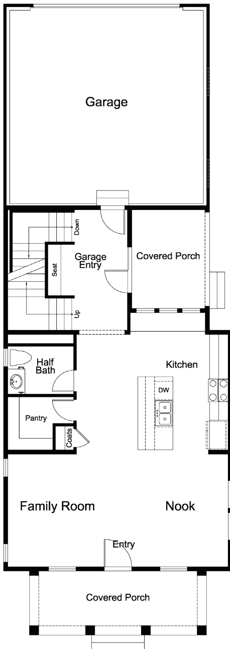
MAIN LEVEL
