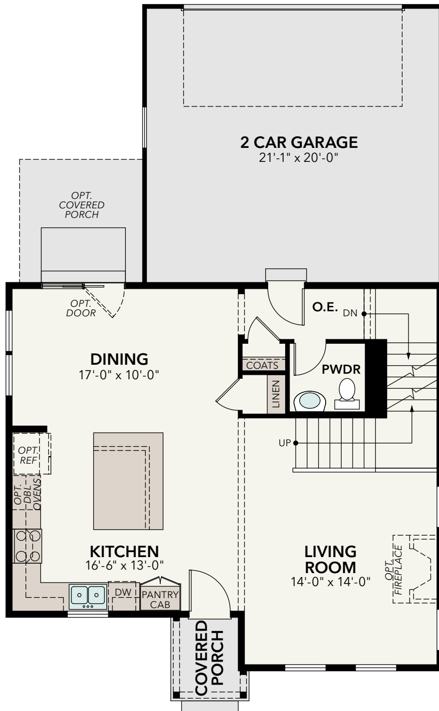
FIRST FLOOR
