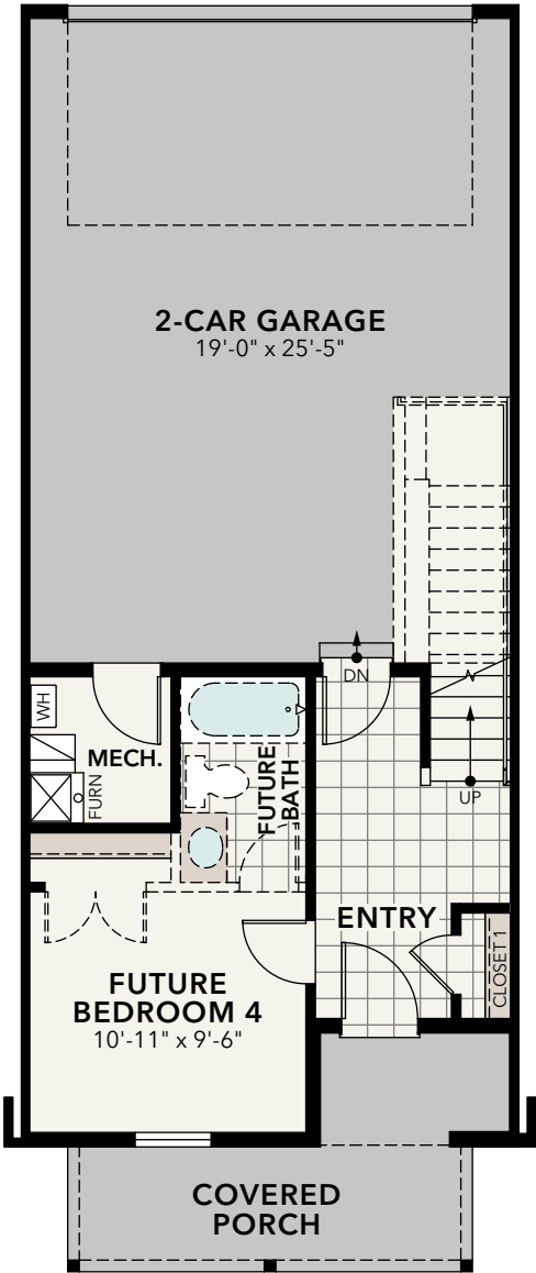
LOWER LEVEL
